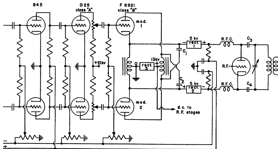
Fig. 11. Cathanode circuit with conventional drive stages.
