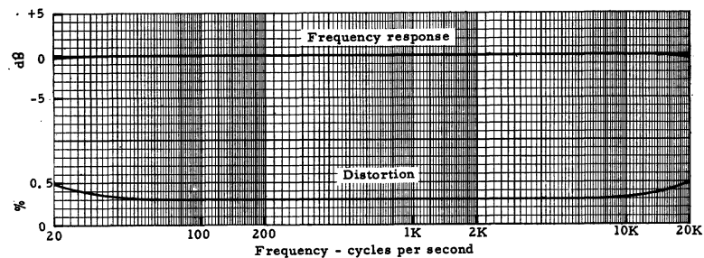
Fig. 14. Response characteristics.
