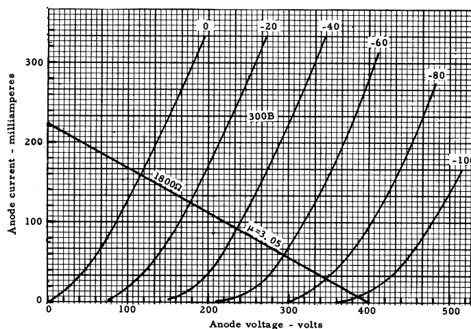
Fig. 4. Anode characteristics W.E. type 300B power triode.
