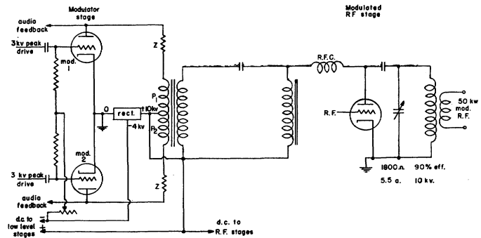
Fig. 1. Conventional high-level modulation circuit.
