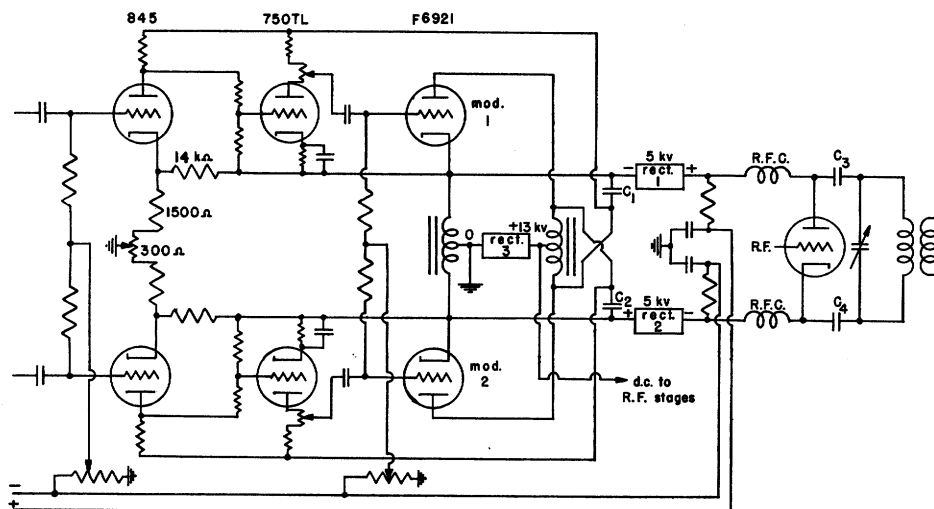
Fig. 12. Cathanode system with floating drive stages.
