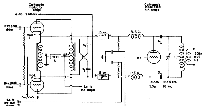
Fig. 2. Cathanode high-level modulation circuit.
