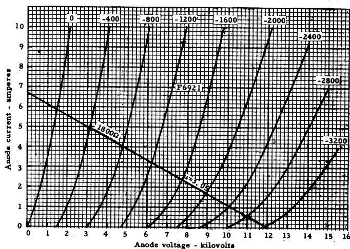
Fig. 3. Anode characteristics ITT type F6921 power triode.
